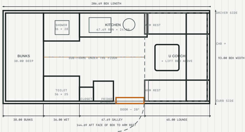
1 — HABITAT PLAN (CURB SIDE BOTTOM, NOSE RIGHT) · SCALE 1:16
